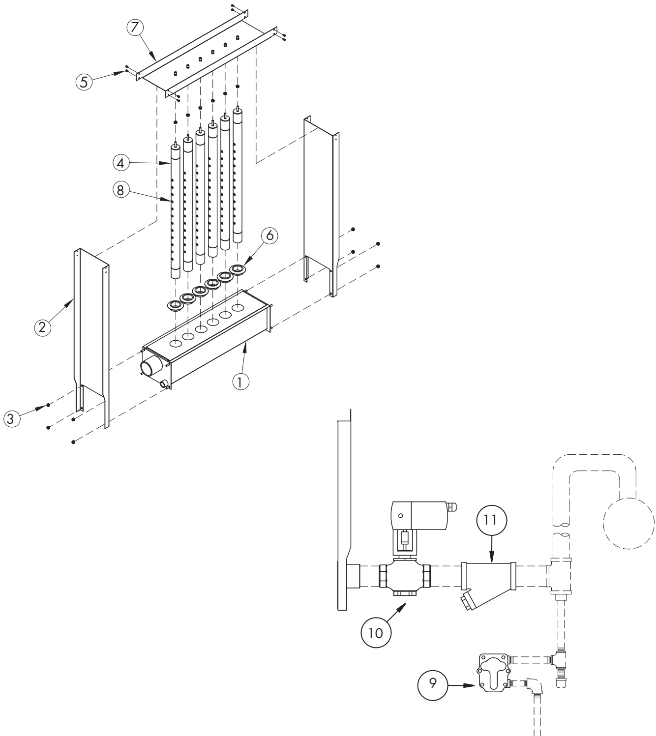
FIGURE 28-1: ULTRA-SORB MODEL MP REPLACEMENT PARTS
